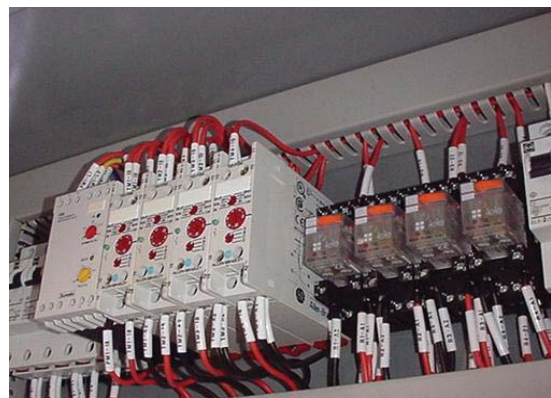
Control & Wiring
